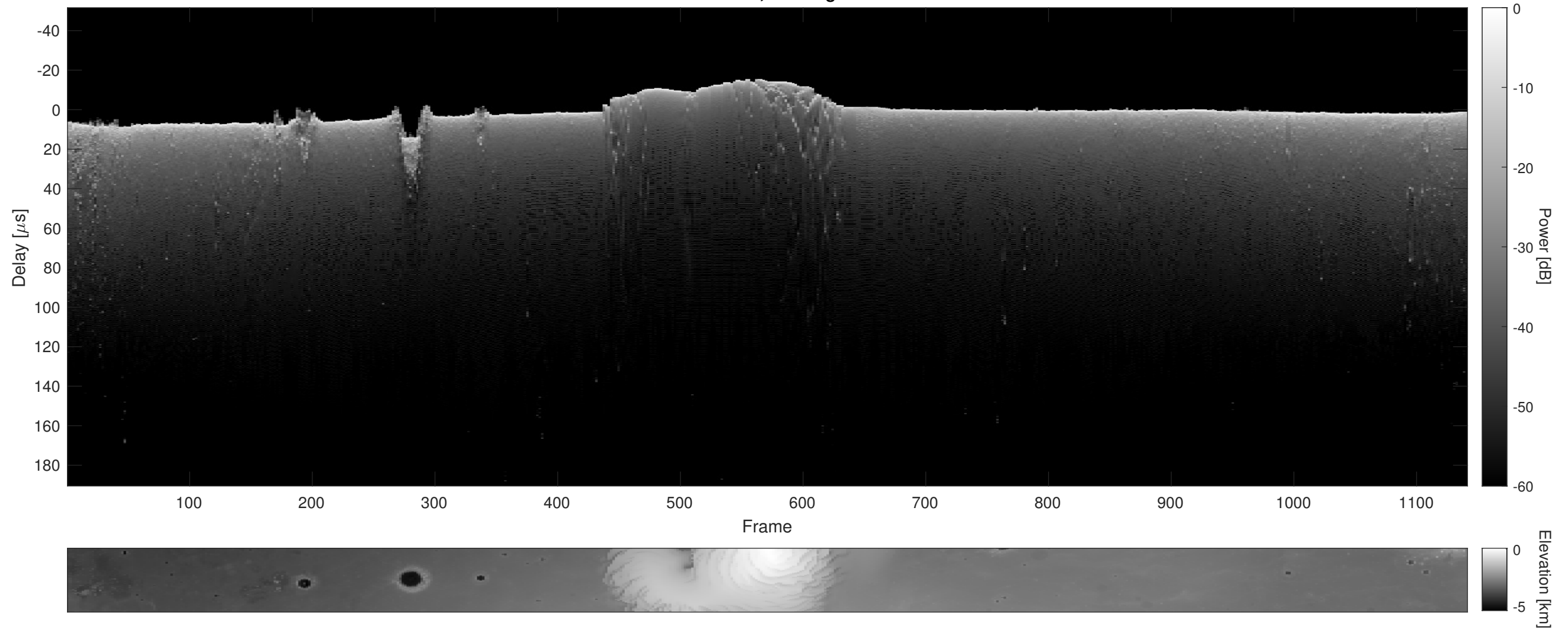
Orbit 11884, Cluttergram
