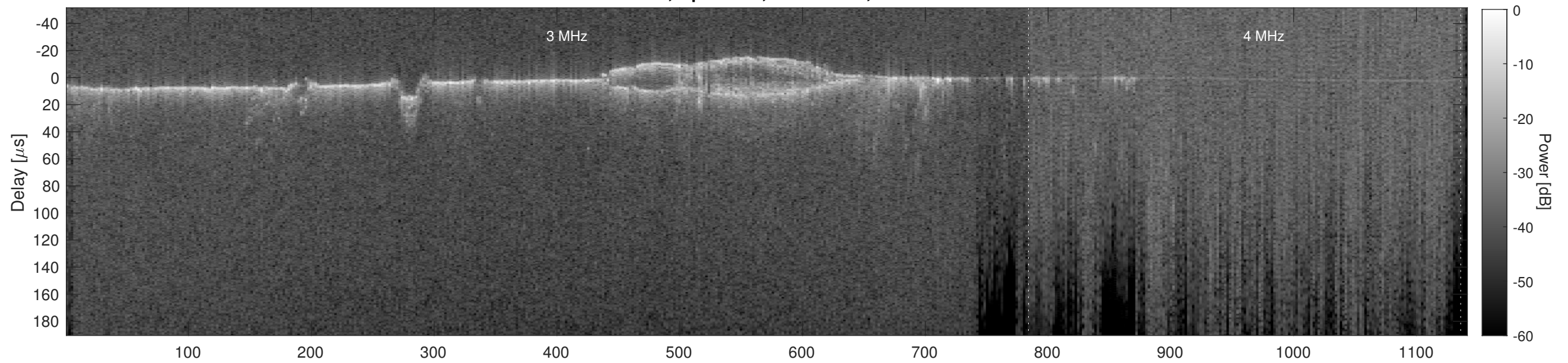
Orbit 11884, Cluttergram
