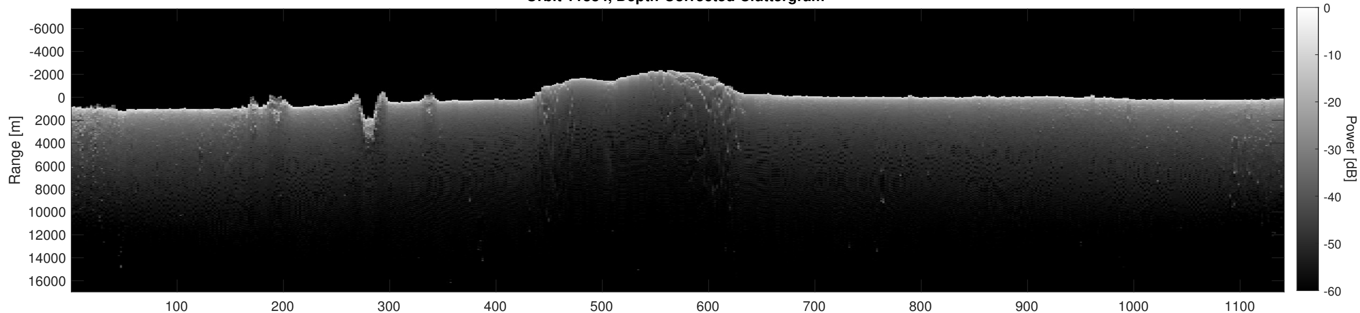
Orbit 11884, Depth-Corrected Cluttergram
