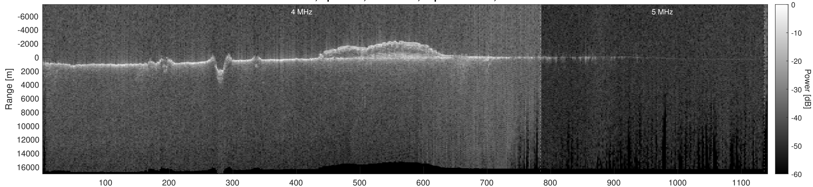
Orbit 11884, Optimized, No Window, Depth-Corrected, Channel 2
