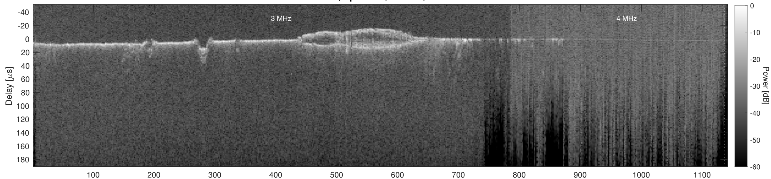
Orbit 11884, Cluttergram
