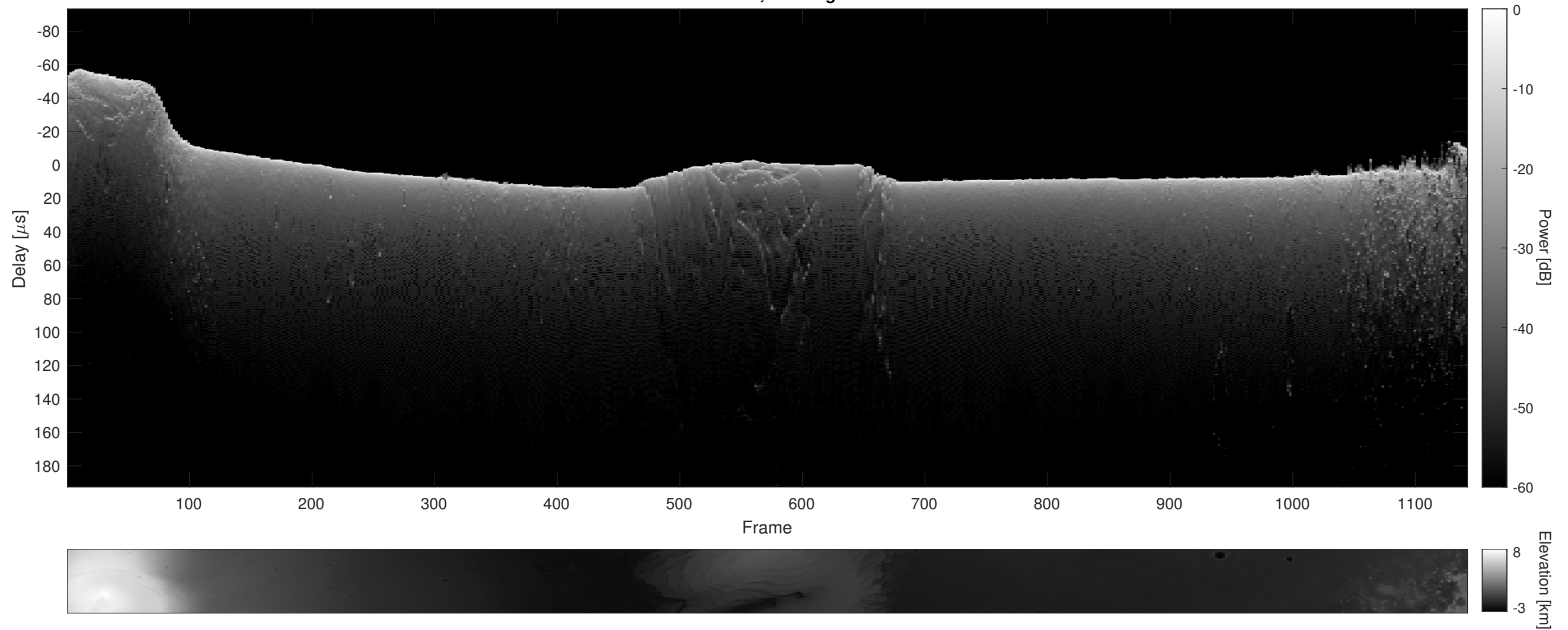
Orbit 11885, Cluttergram
