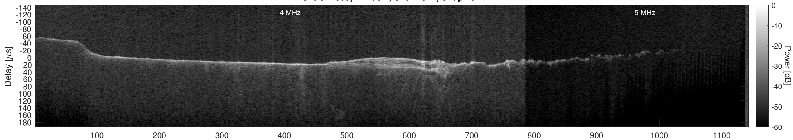
Orbit 11885, Window, Channel 1, Optimized
