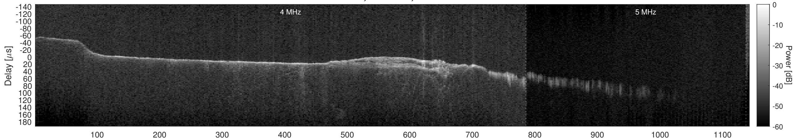
Orbit 11885, Window, Channel 1, Chapman
