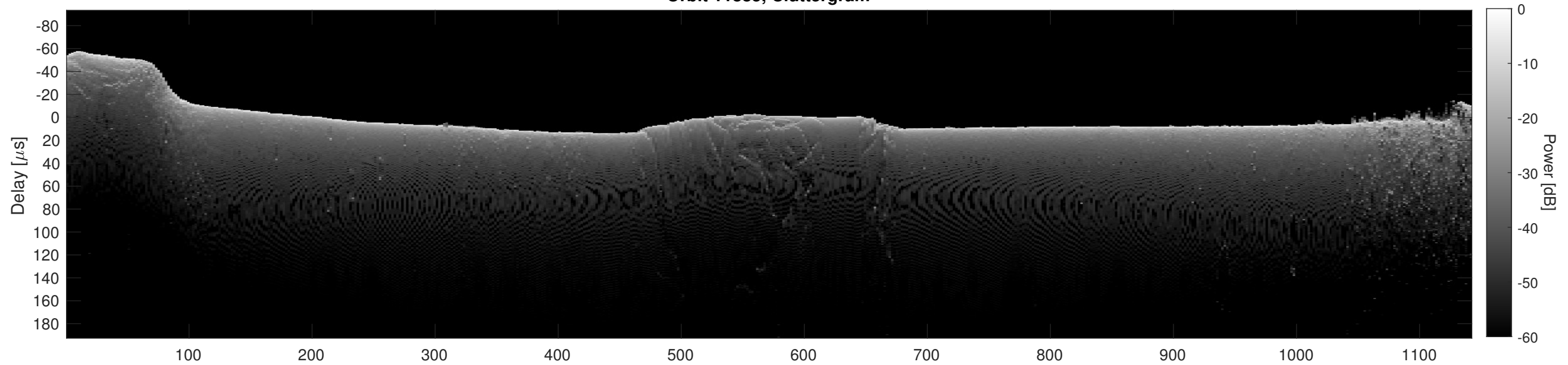
Orbit 11885, Cluttergram
