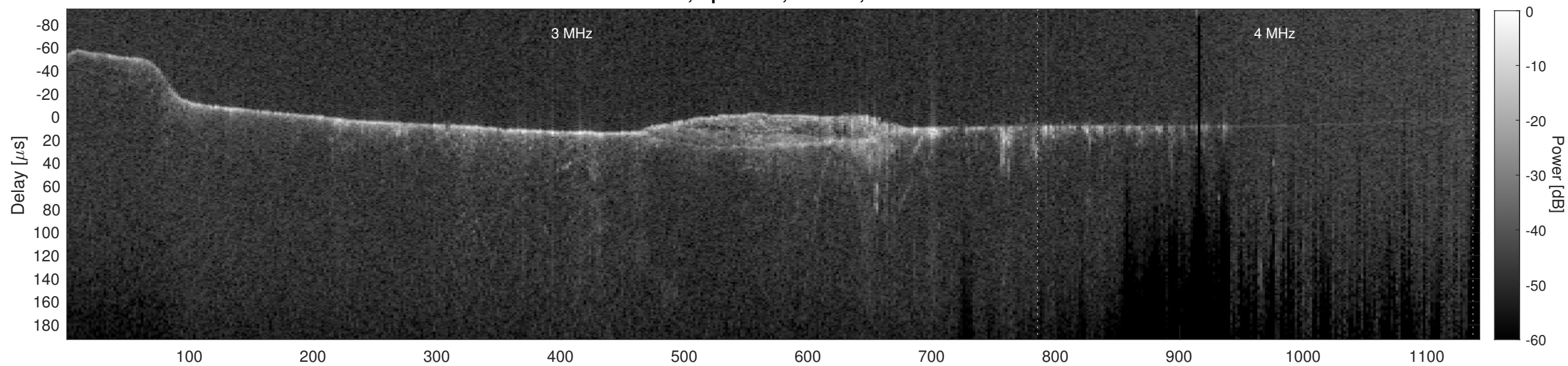
Orbit 11885, Cluttergram
