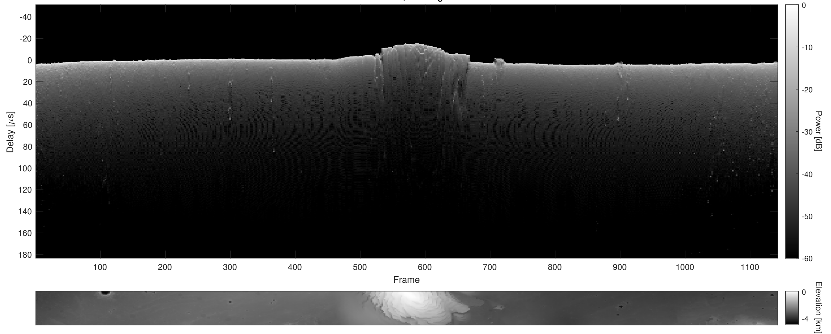
Orbit 11886, Cluttergram
