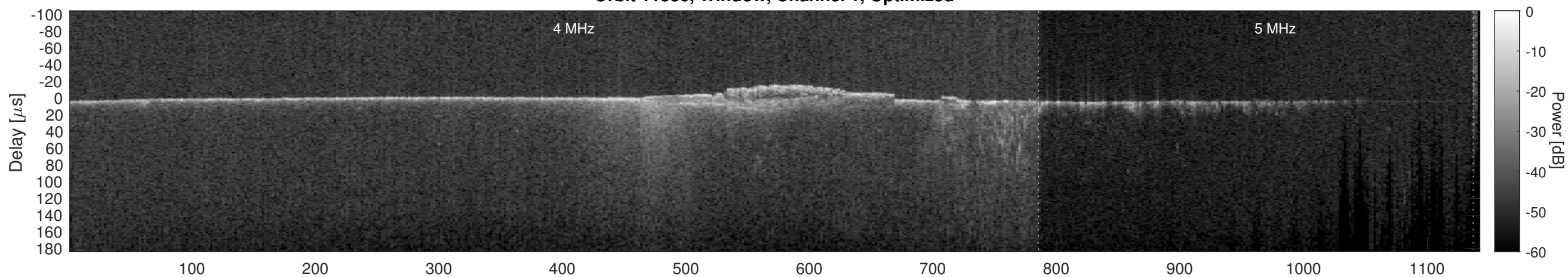
Orbit 11886, Cluttergram
