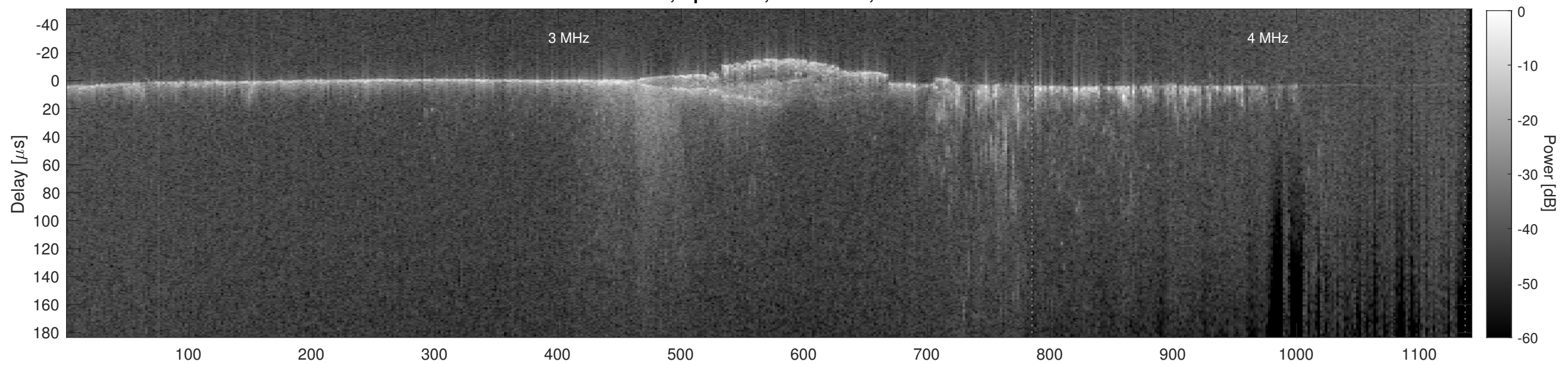
Orbit 11886, Cluttergram
