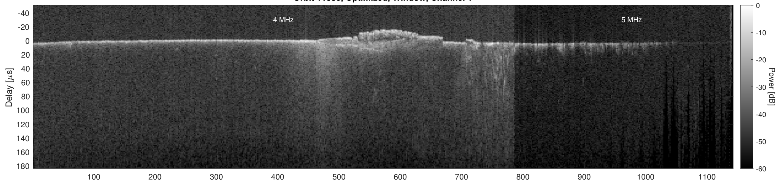
Orbit 11886, Optimized, Window, Channel 2
