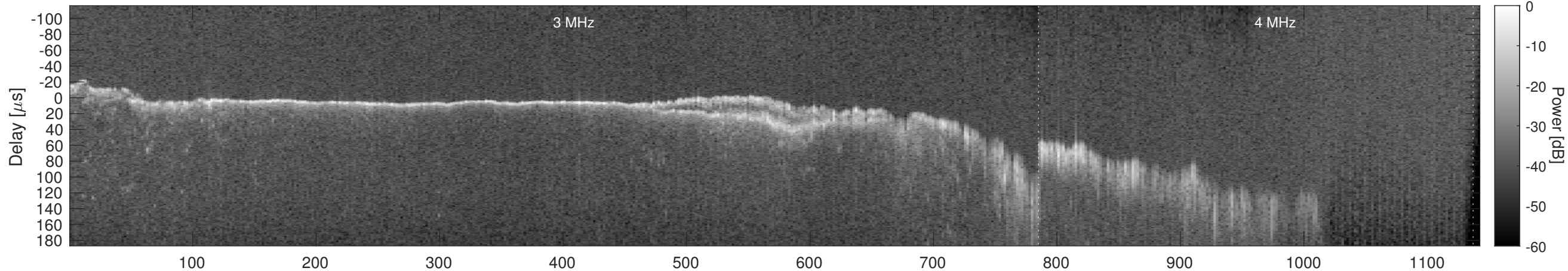
Orbit 11887, Window, Channel 2, Chapman
