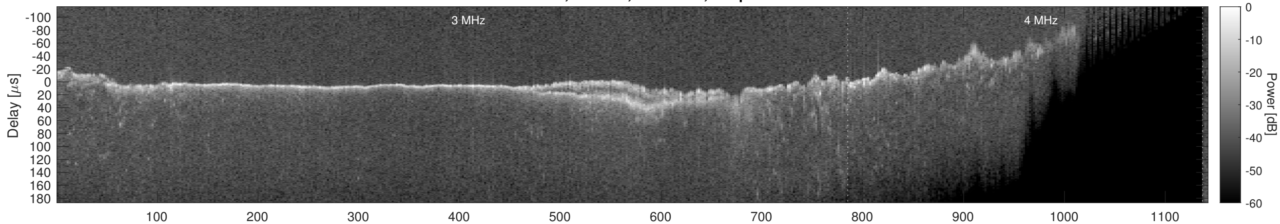
Orbit 11887, Window, Channel 2, Optimized
