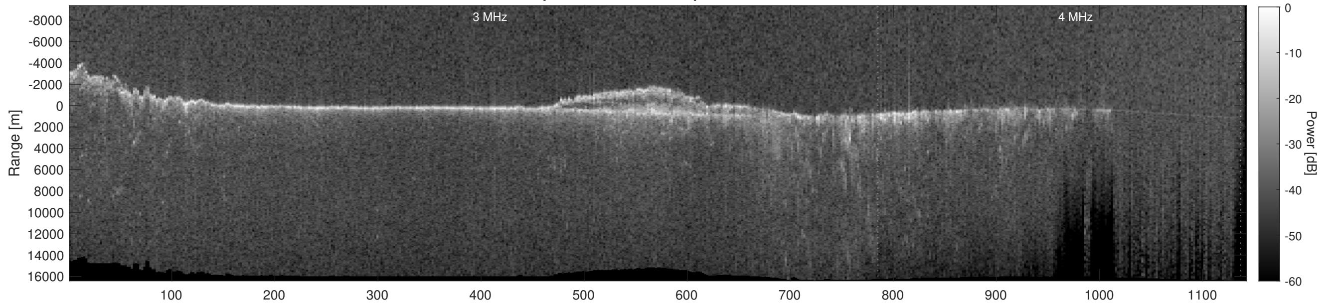
Orbit 11887, Depth-Corrected Cluttergram
