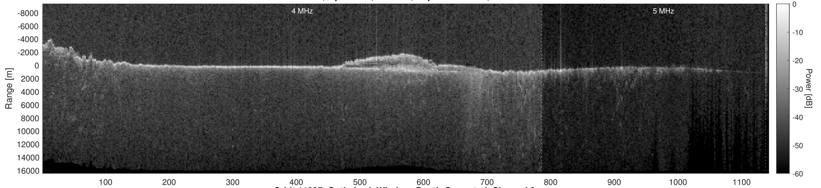
Orbit 11887, Optimized, Window, Depth-Corrected, Channel 2
