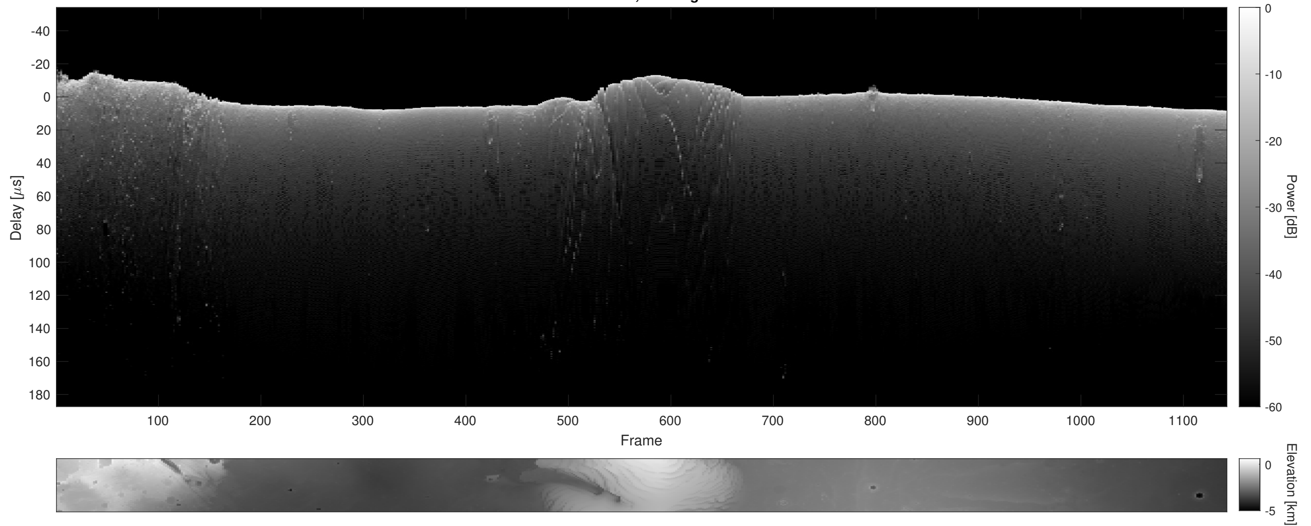
Orbit 11888, Cluttergram
