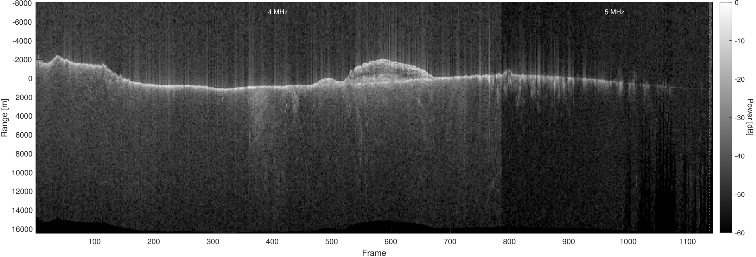
Orbit 11888, Optimized, No Window, Depth-Corrected, Channel 2
