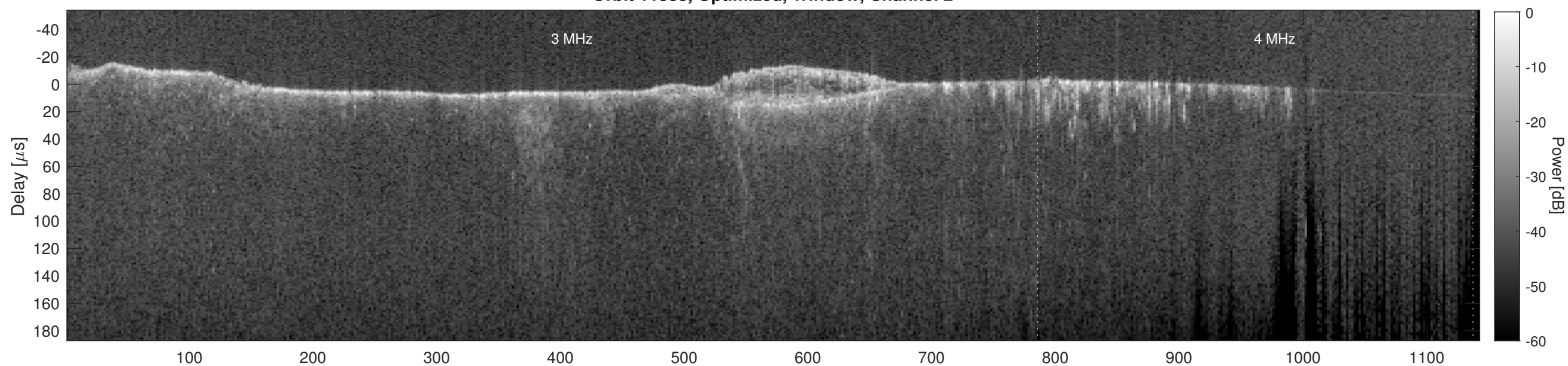
Orbit 11888, Cluttergram
