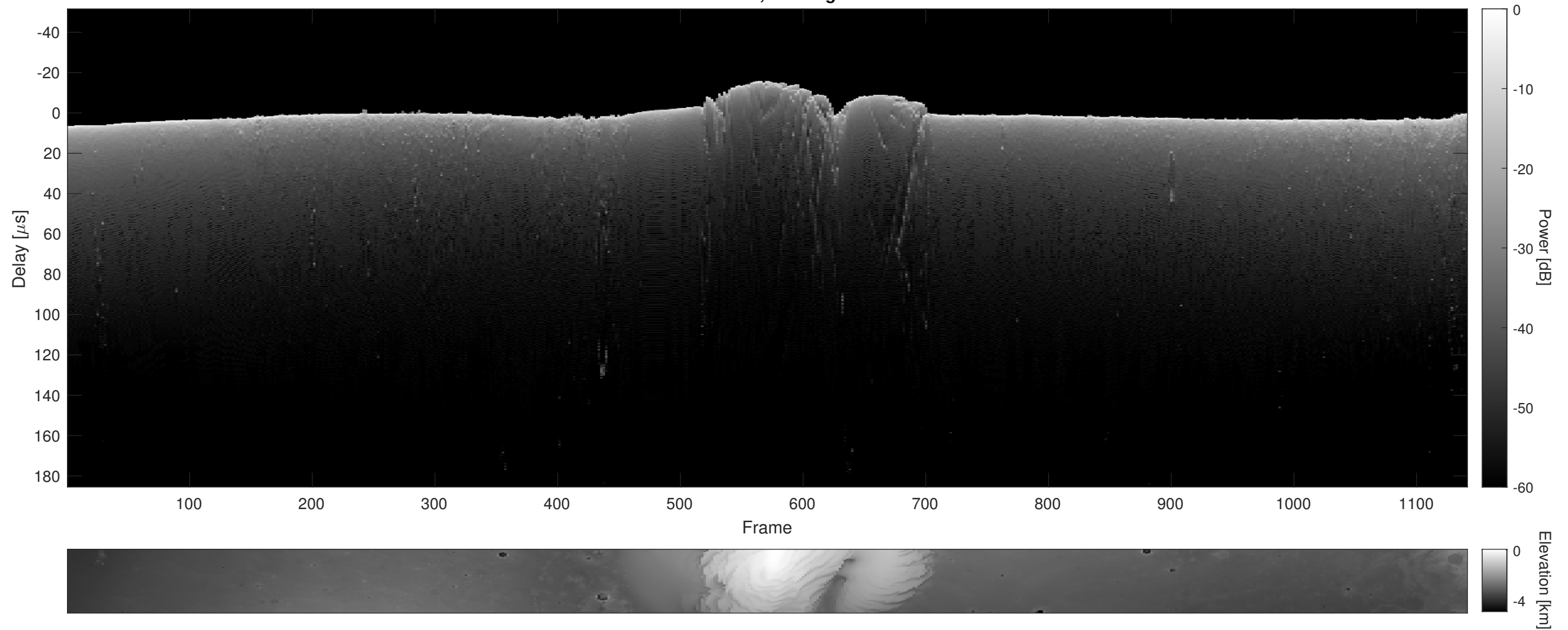
Orbit 11889, Cluttergram
