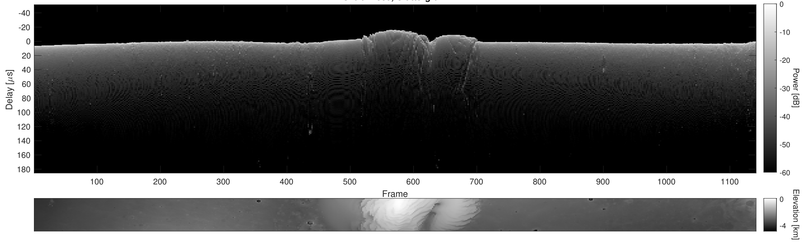
Orbit 11889, Cluttergram
