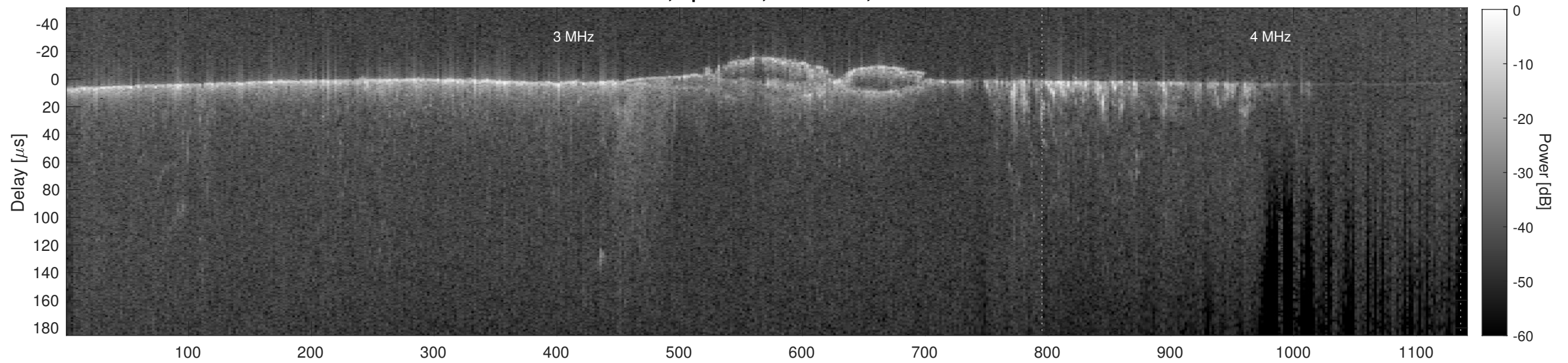
Orbit 11889, Cluttergram
