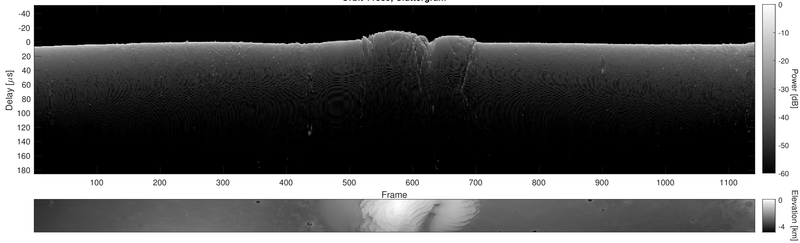
Orbit 11889, Cluttergram
