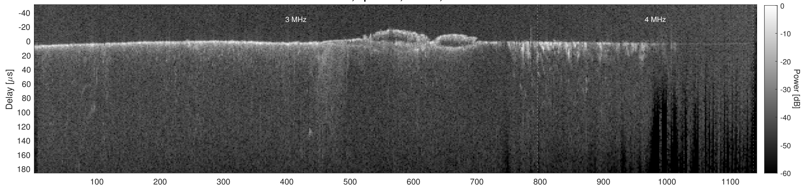
Orbit 11889, Cluttergram
