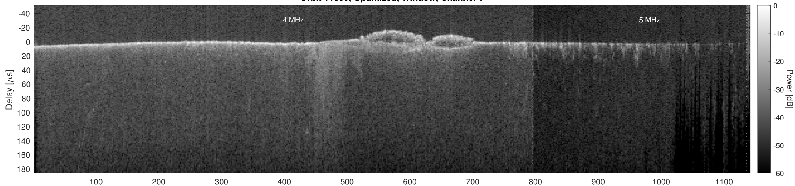
Orbit 11889, Optimized, Window, Channel 2
