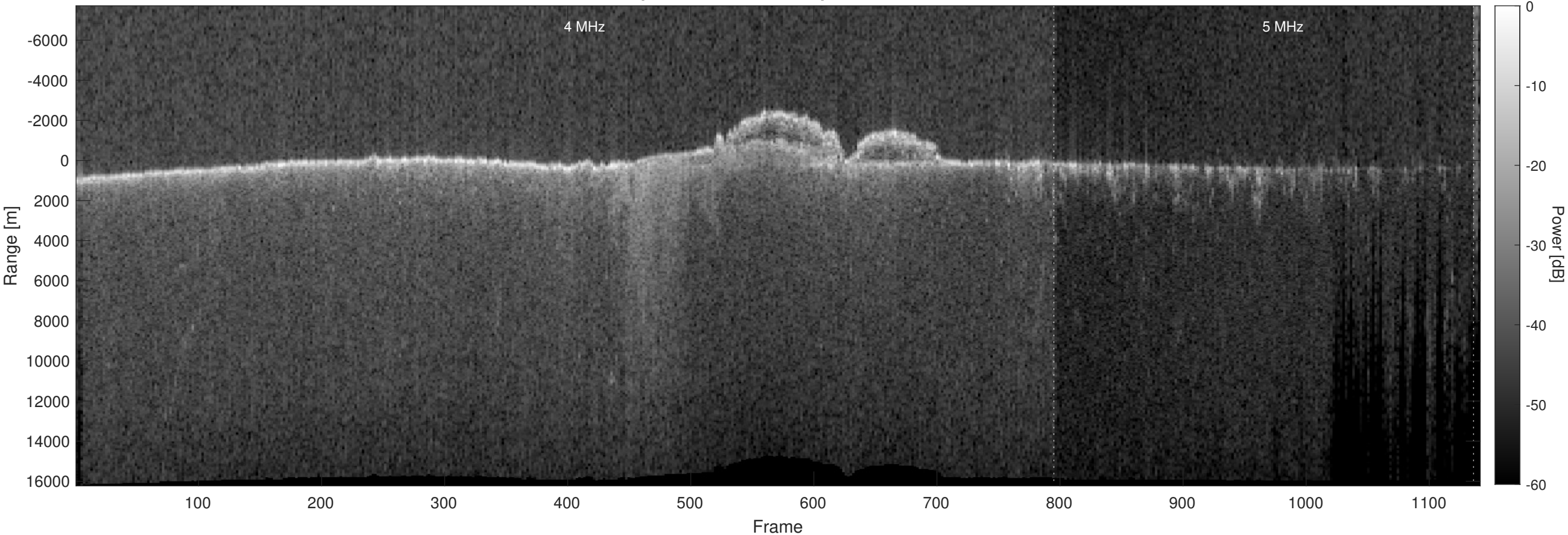
Orbit 11889, Optimized, Window, Depth-Corrected, Channel 2
