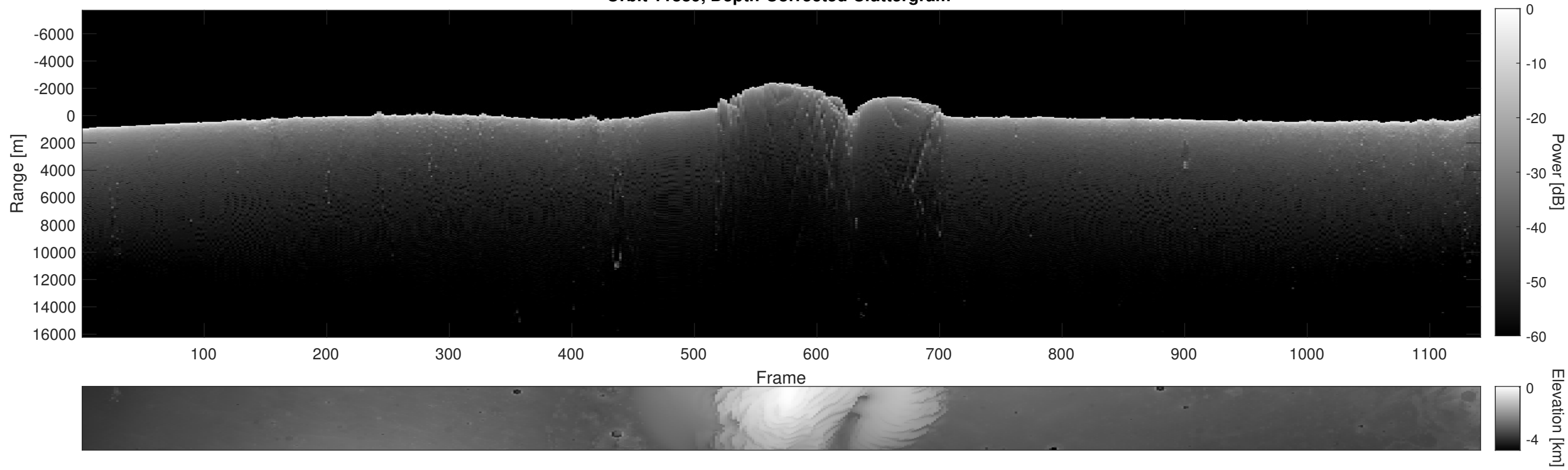
Orbit 11889, Depth-Corrected Cluttergram
