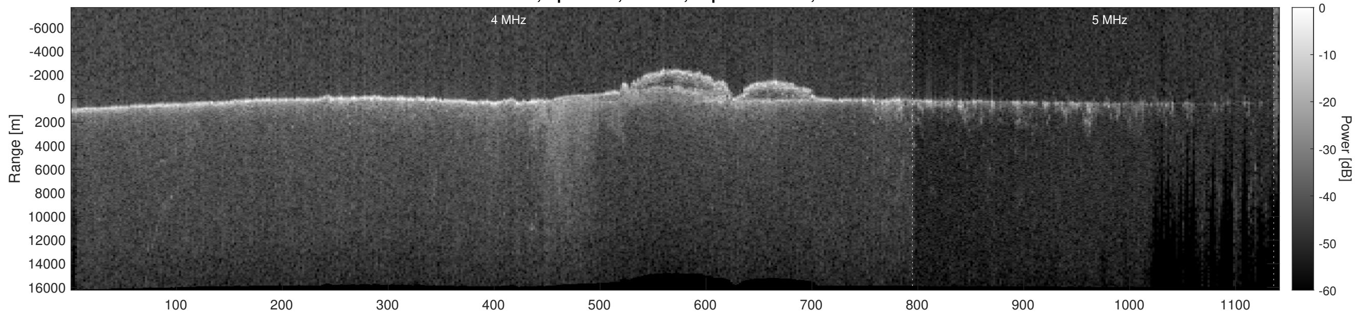
Orbit 11889, Optimized, Window, Depth-Corrected, Channel 2
