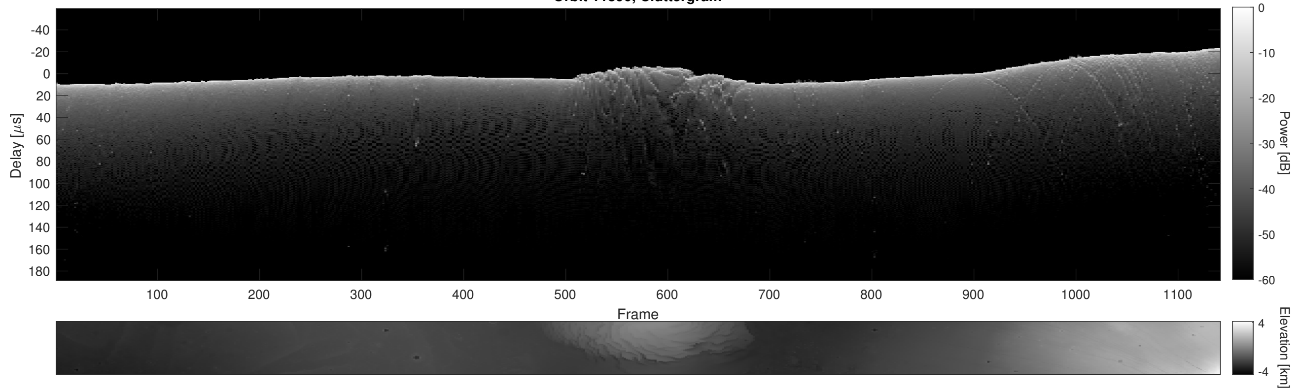
Orbit 11890, Cluttergram
