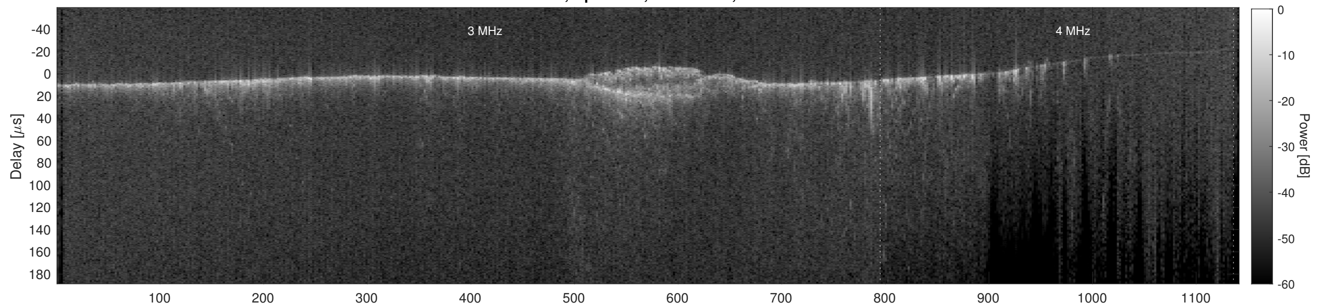
Orbit 11890, Cluttergram
