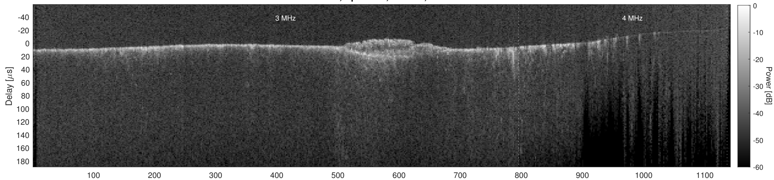
Orbit 11890, Cluttergram
