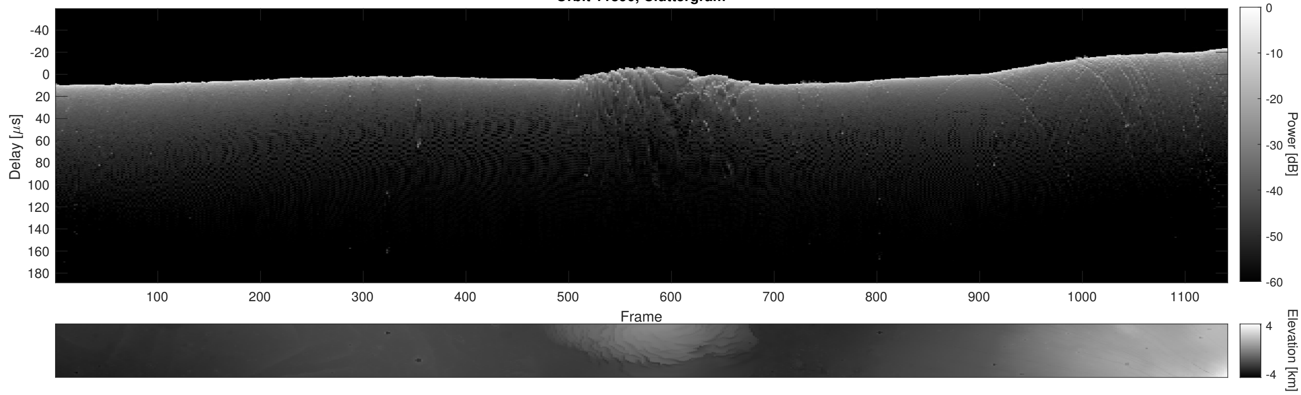
Orbit 11890, Cluttergram
