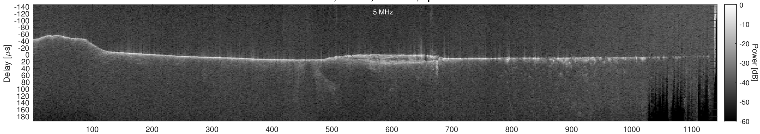
Orbit 11892, Cluttergram
