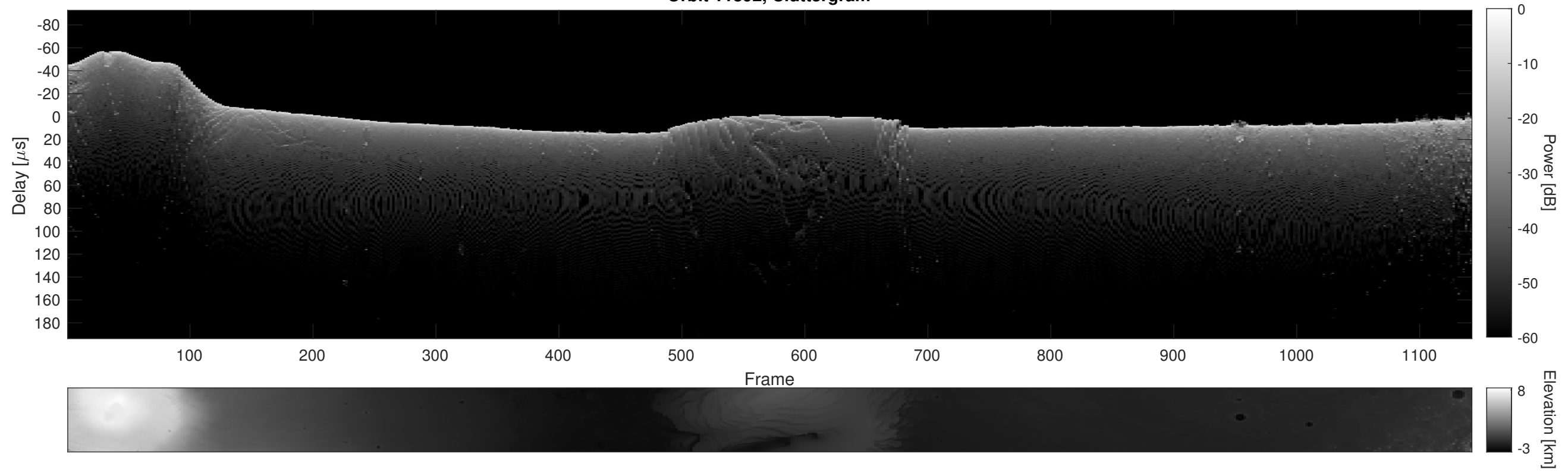
Orbit 11892, Cluttergram
