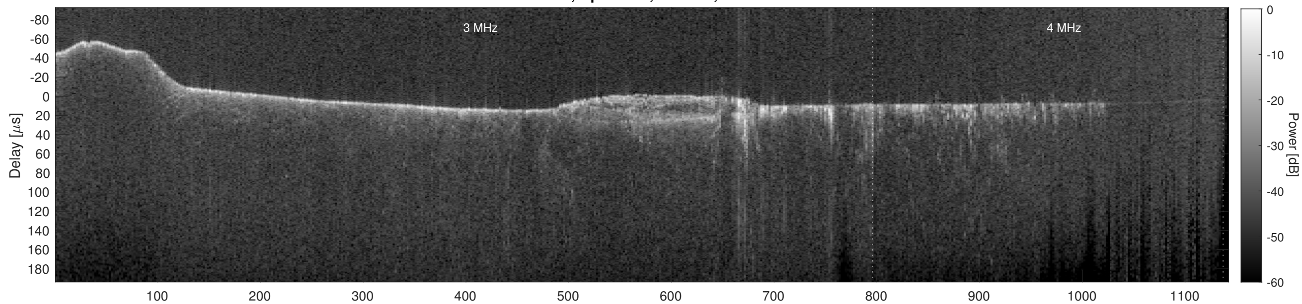
Orbit 11892, Cluttergram
