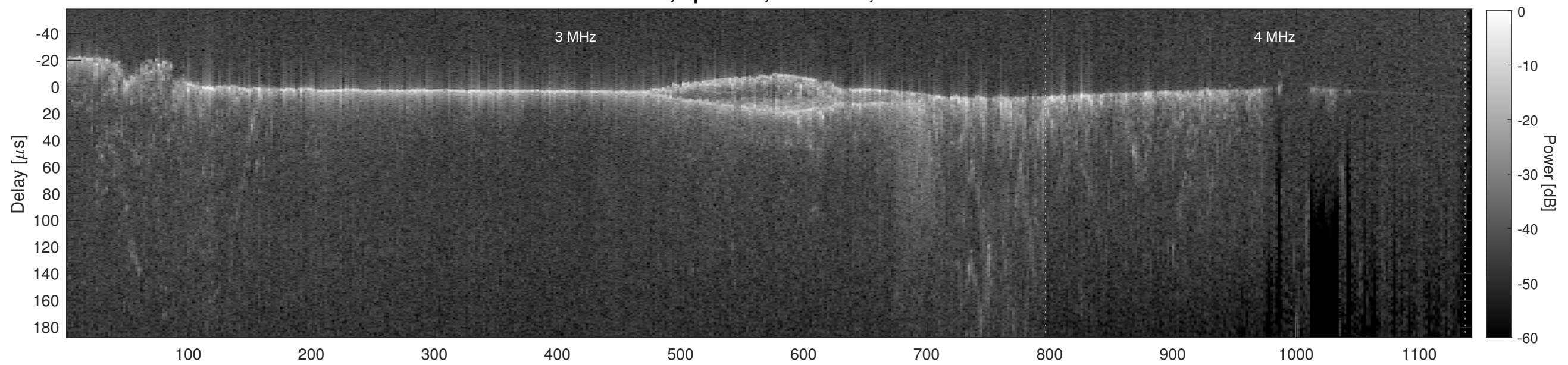
Orbit 11894, Cluttergram
