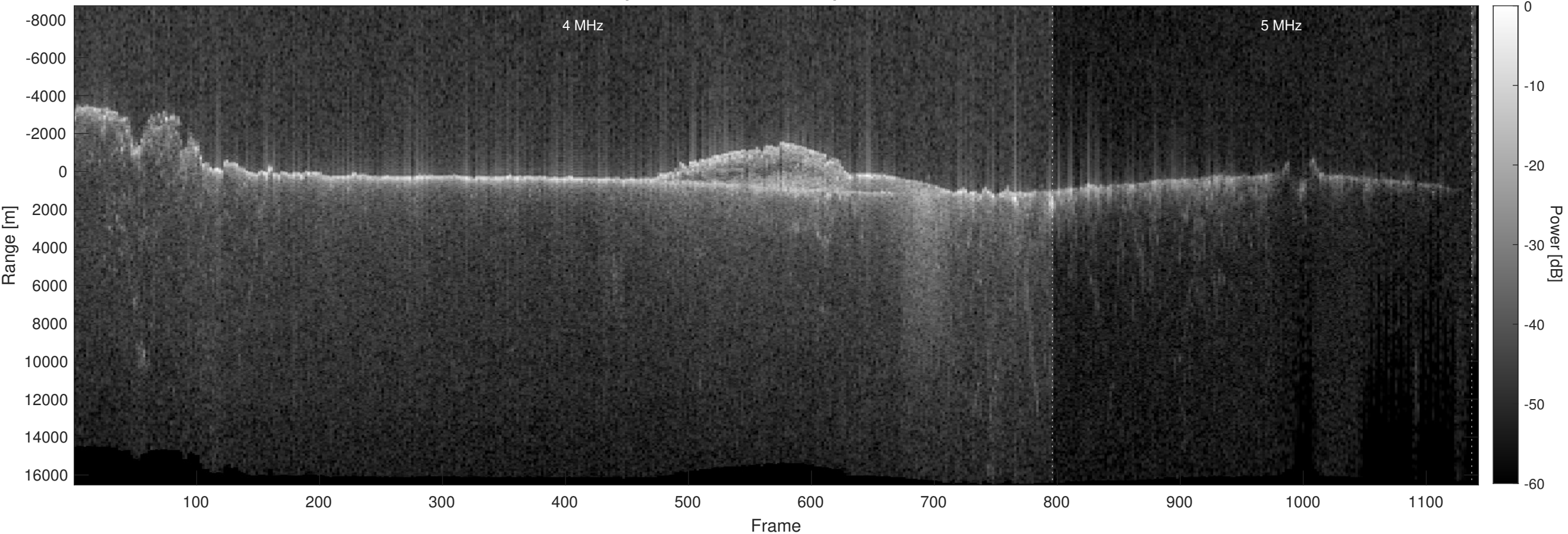
Orbit 11894, Optimized, No Window, Depth-Corrected, Channel 2
