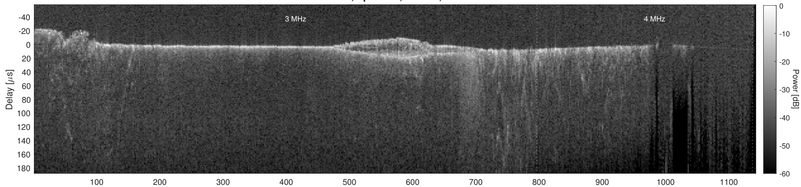
Orbit 11894, Cluttergram
