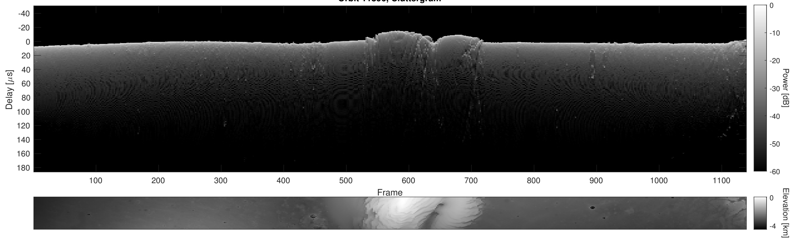
Orbit 11896, Cluttergram
