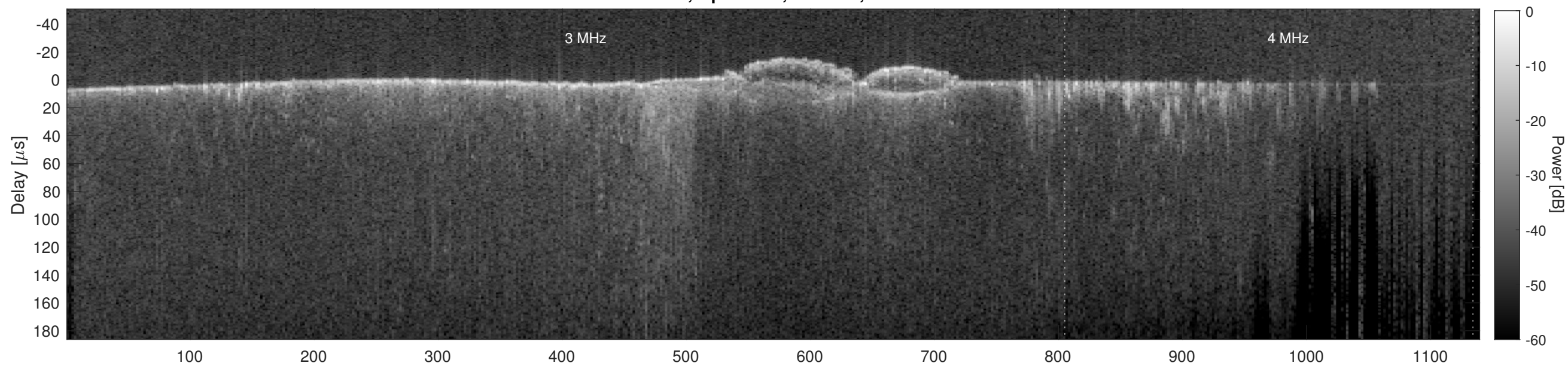
Orbit 11896, Cluttergram
