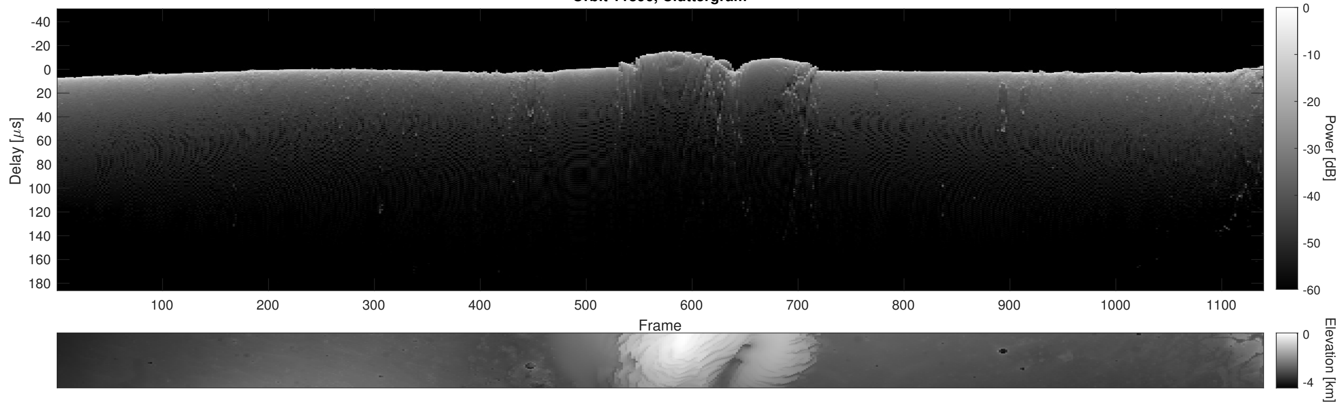
Orbit 11896, Cluttergram
