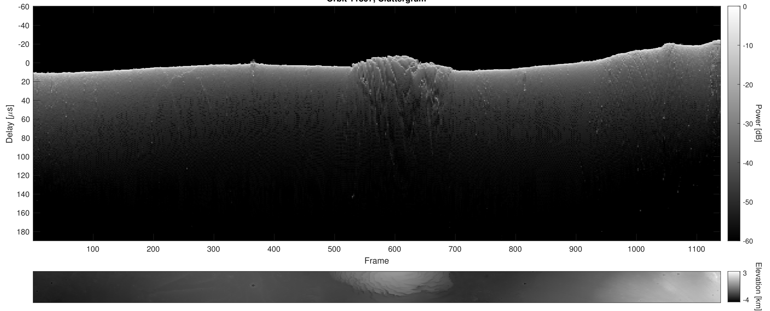
Orbit 11897, Cluttergram
