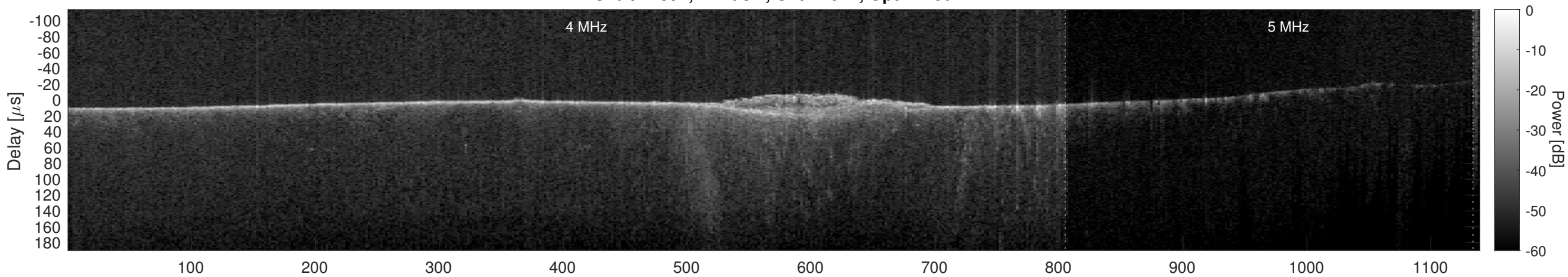
Orbit 11897, Cluttergram
