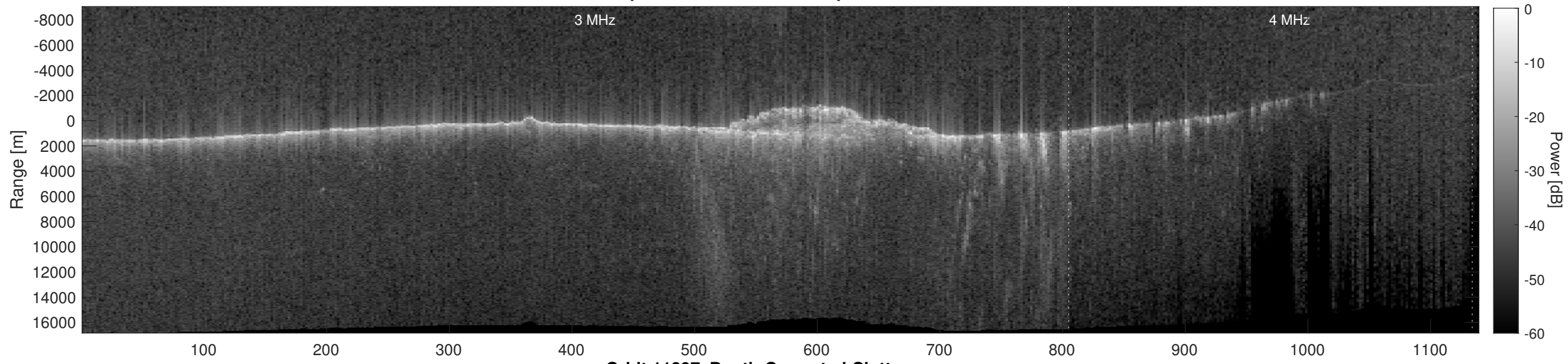
Orbit 11897, Depth-Corrected Cluttergram
