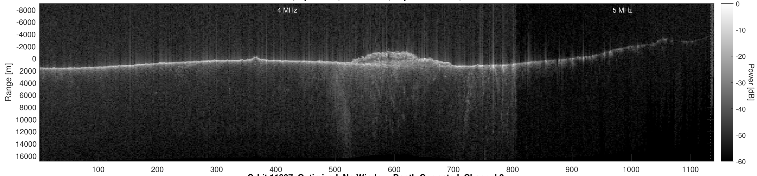
Orbit 11897, Optimized, No Window, Depth-Corrected, Channel 2
