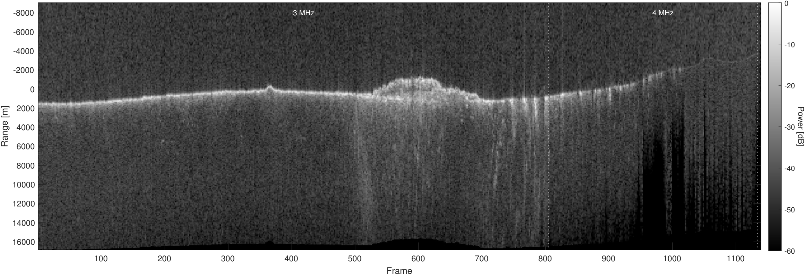
Orbit 11897, Optimized, Window, Depth-Corrected, Channel 2
