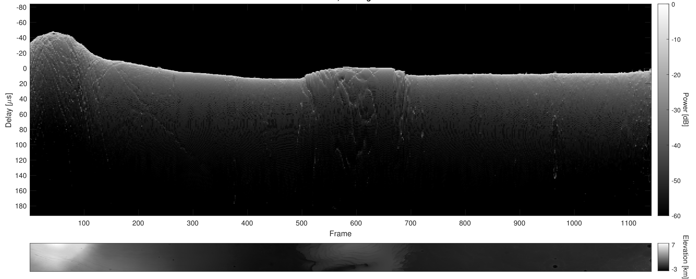
Orbit 11899, Cluttergram
