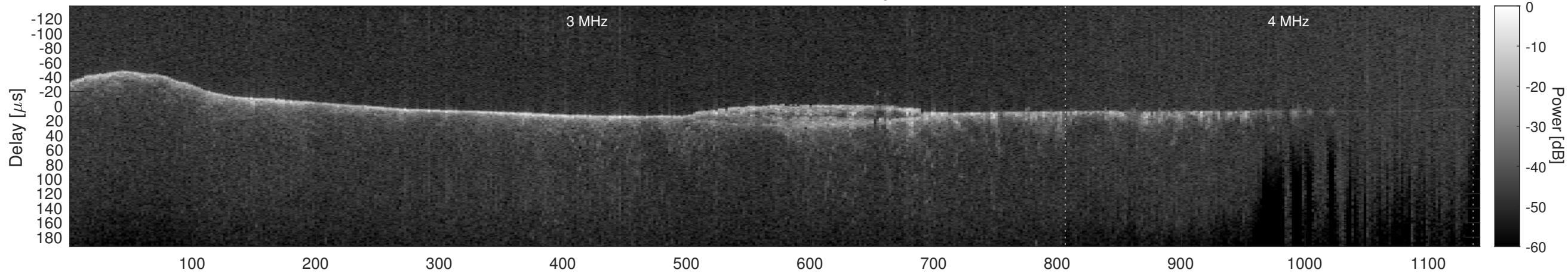
Orbit 11899, Cluttergram
