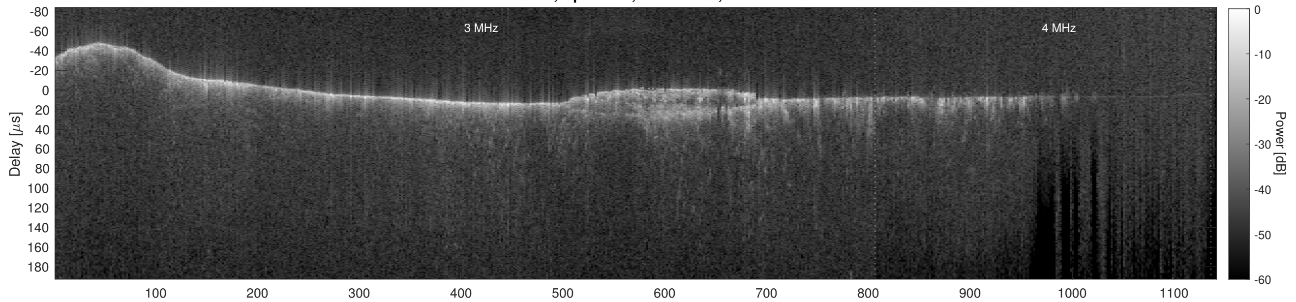
Orbit 11899, Cluttergram
