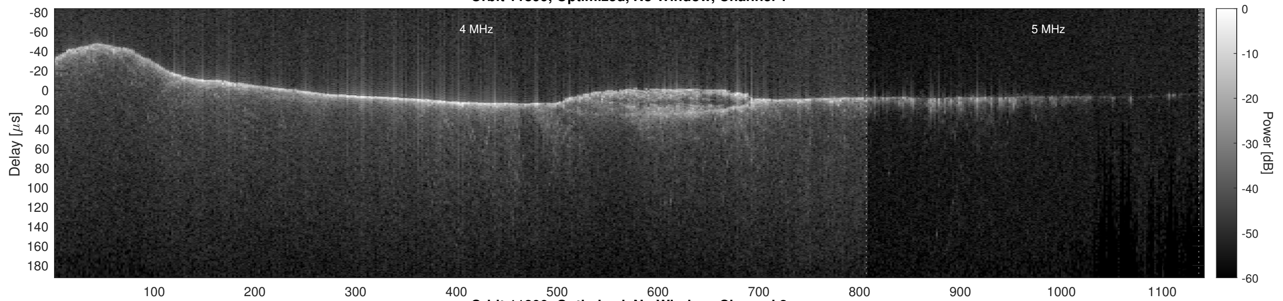
Orbit 11899, Optimized, No Window, Channel 2
