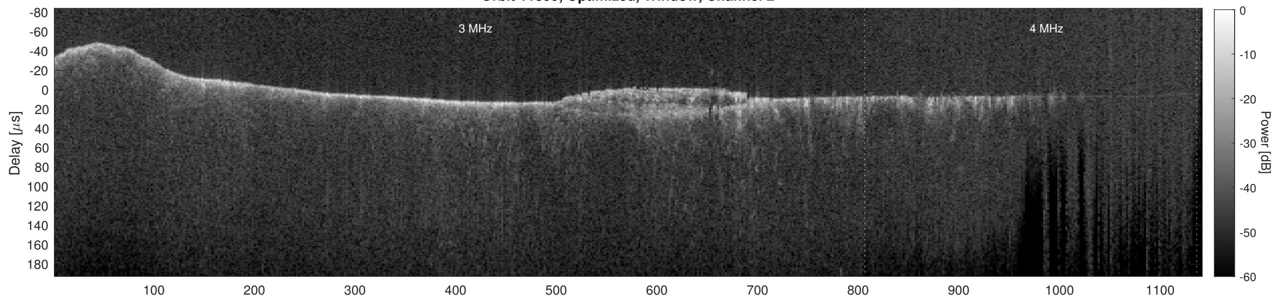
Orbit 11899, Cluttergram
