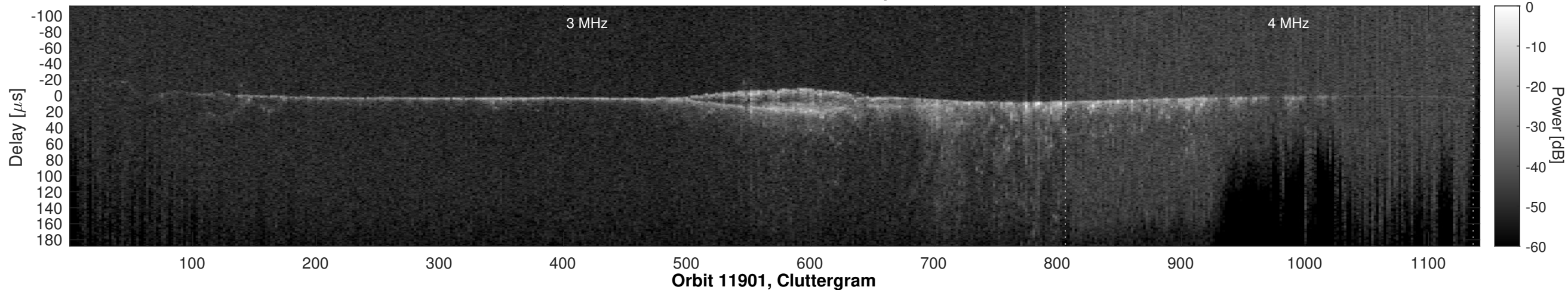
Orbit 11901, Window, Channel 2, Optimized
