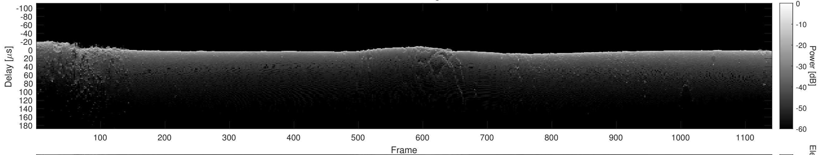
Orbit 11901, Cluttergram
