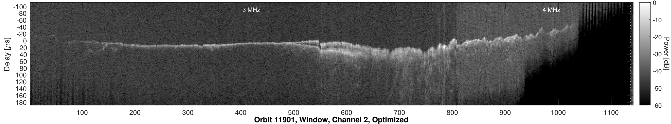
Orbit 11901, Window, Channel 2, Chapman
