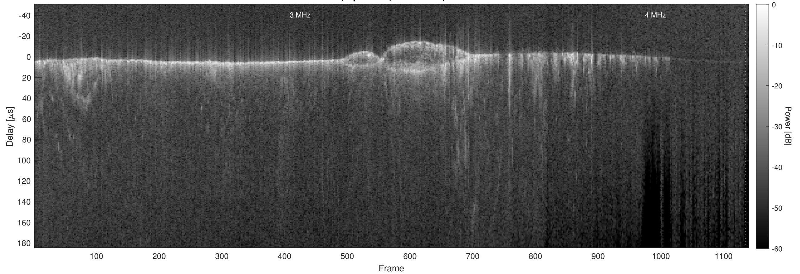
Orbit 11902, Optimized, No Window, Channel 2
