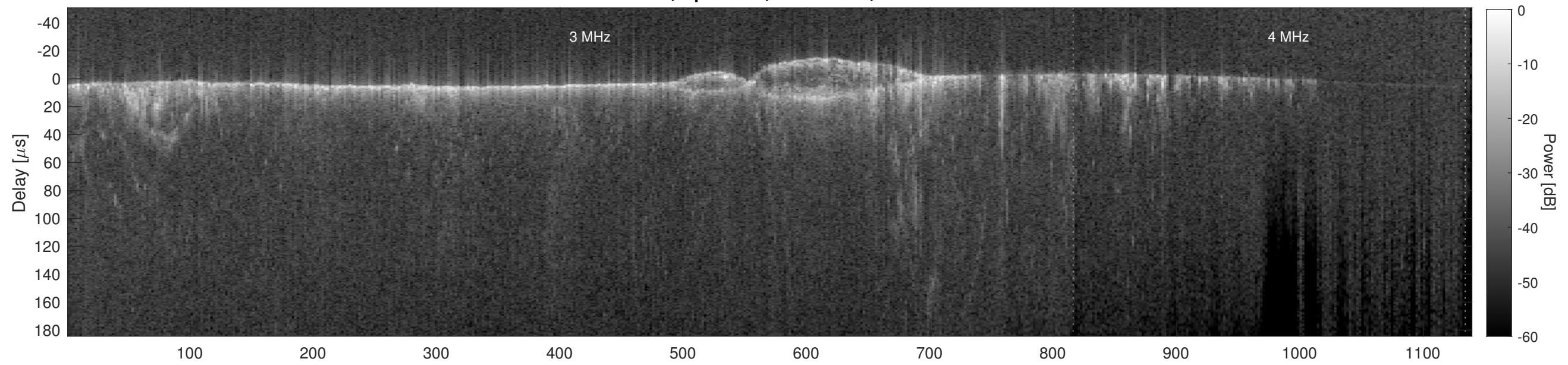
Orbit 11902, Cluttergram
