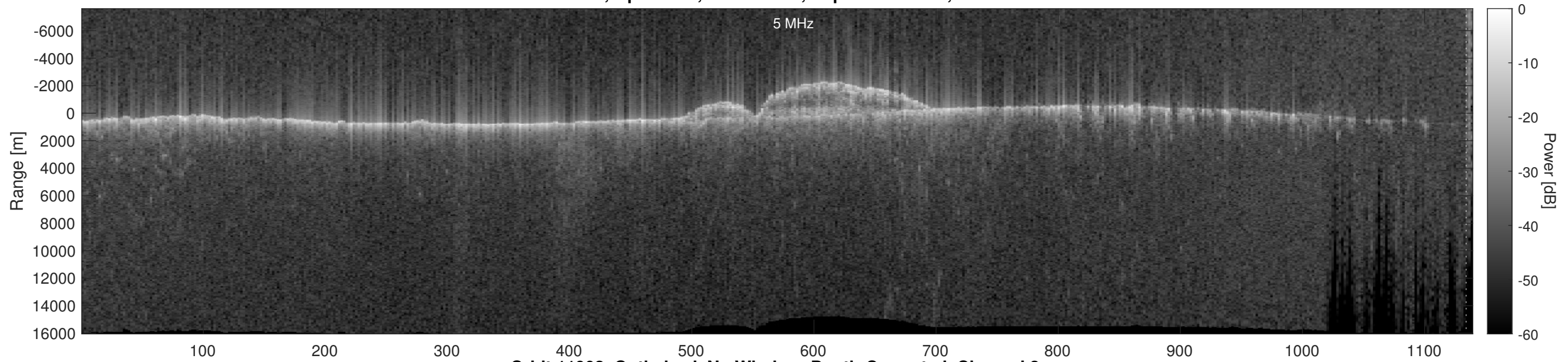
Orbit 11902, Optimized, No Window, Depth-Corrected, Channel 2
