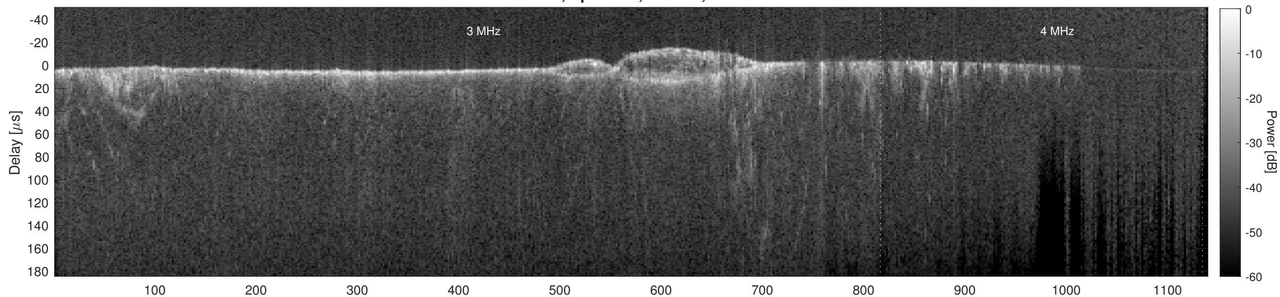
Orbit 11902, Cluttergram
