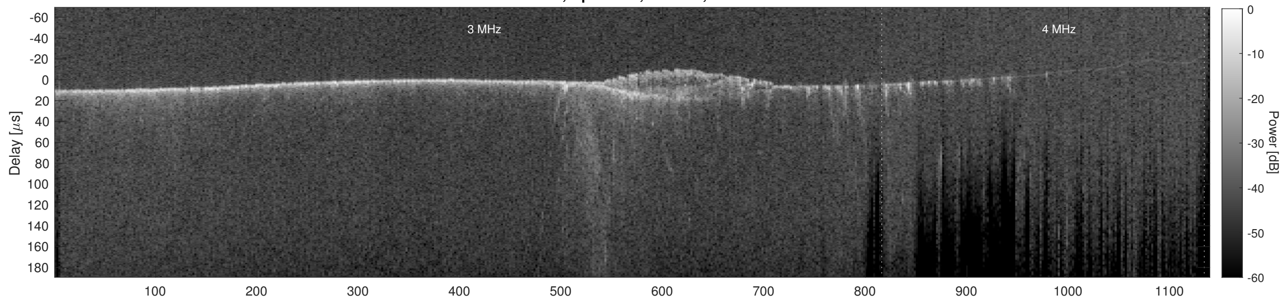
Orbit 11904, Cluttergram
