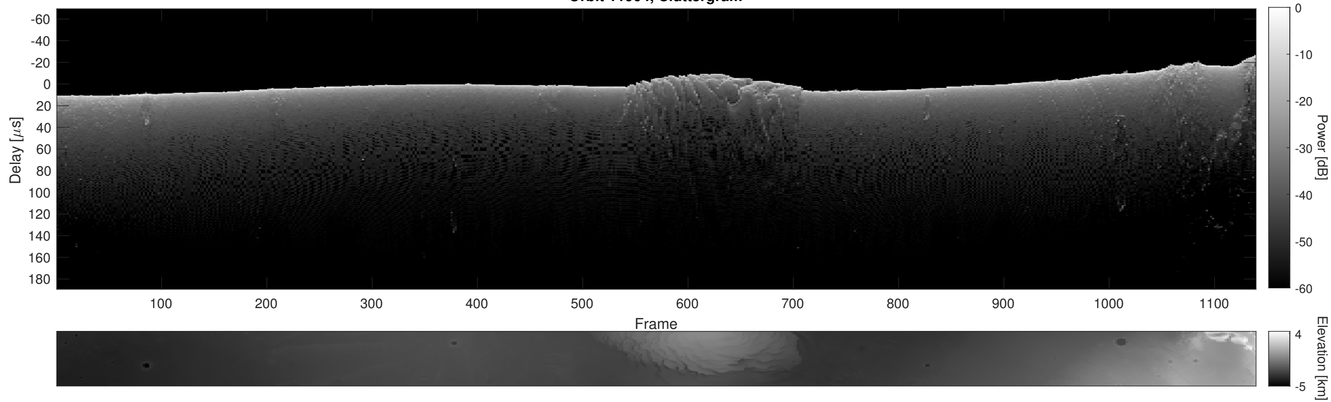
Orbit 11904, Cluttergram
