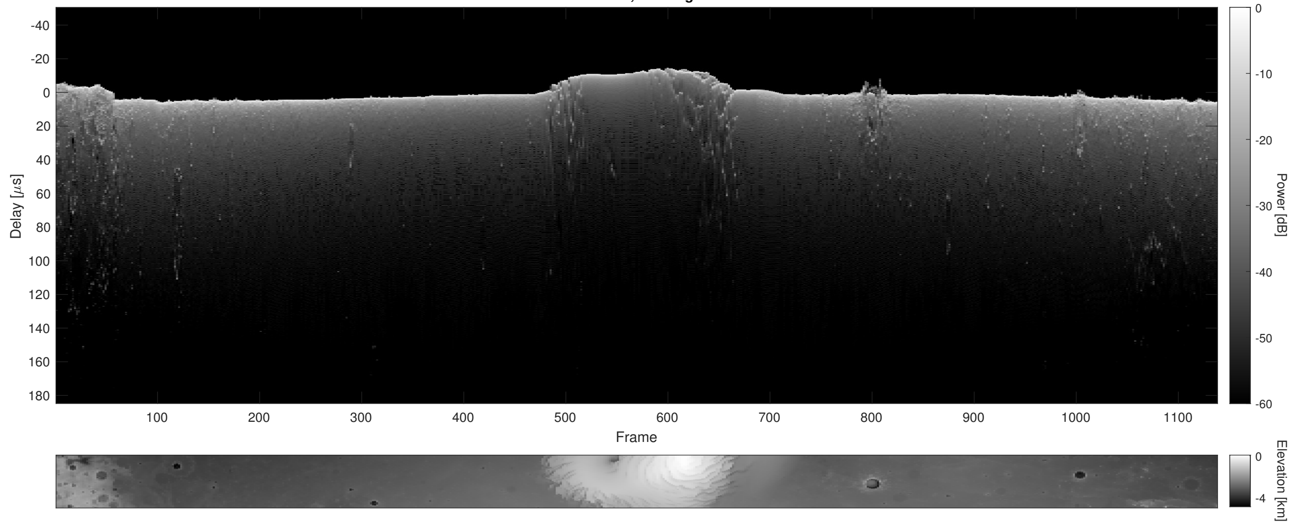
Orbit 11905, Cluttergram
