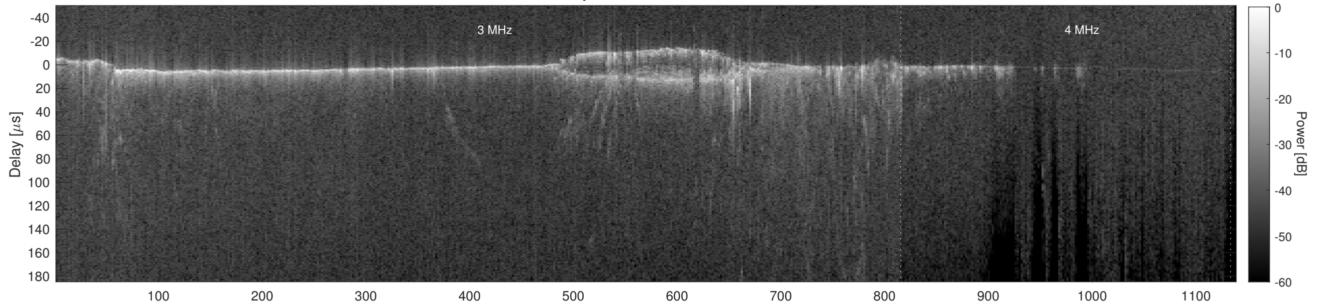
Orbit 11905, Cluttergram
