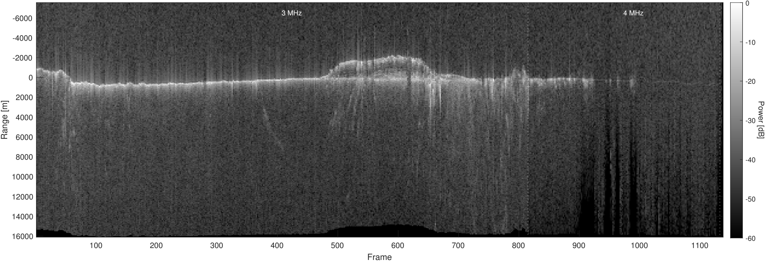
Orbit 11905, Optimized, No Window, Depth-Corrected, Channel 2
