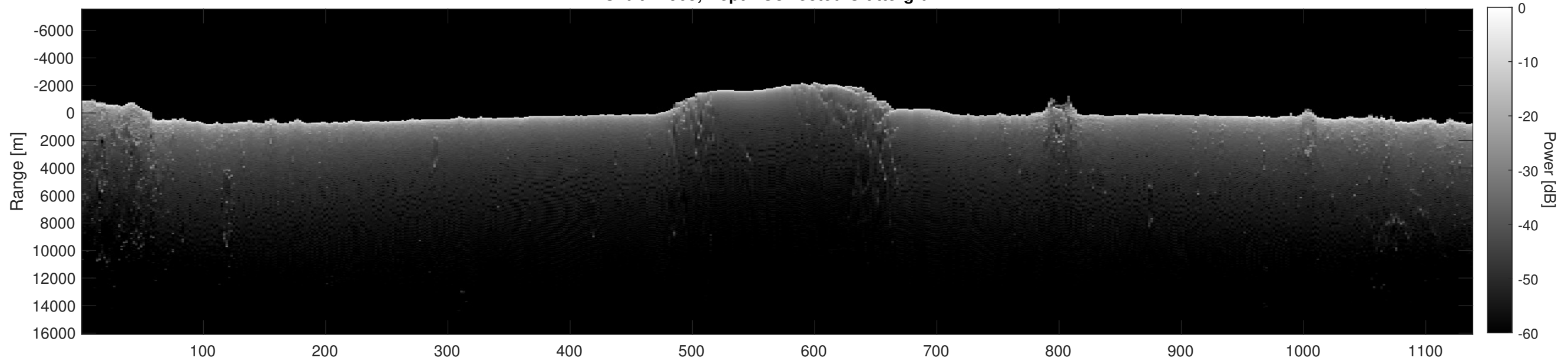
Orbit 11905, Depth-Corrected Cluttergram
