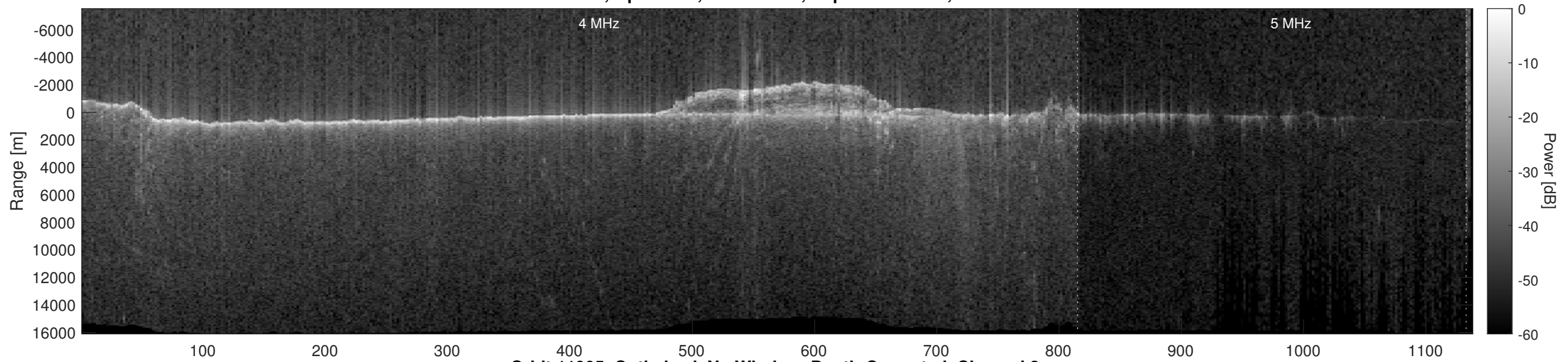
Orbit 11905, Optimized, No Window, Depth-Corrected, Channel 2
